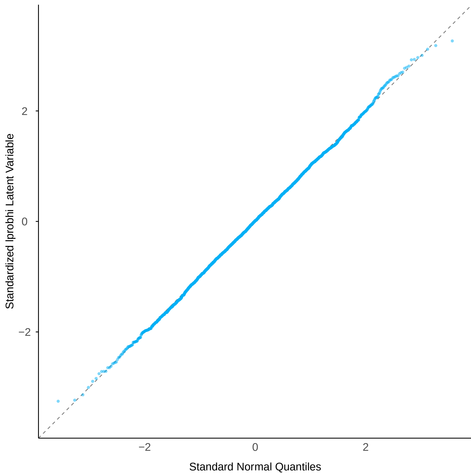
Normal Q-Q: Iprobhi Latent Variable
